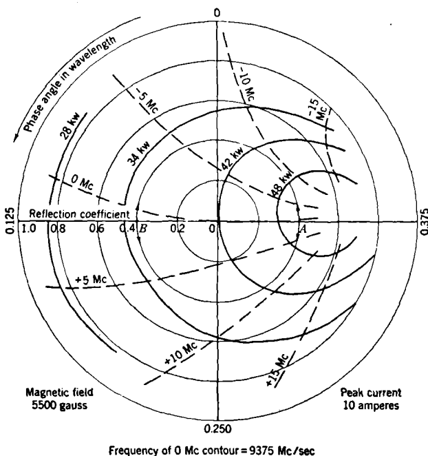
FIG. 1-32.—Typical Rieke diagram (725).
